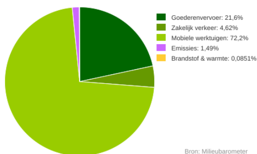
Mechielsen Oldehove 2016 - CO 2 -meter
